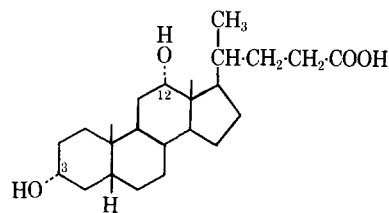
34. Deoxycholic acid
