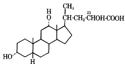
35. Bitocholeic acid
