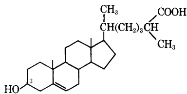
18. 3 \beta -Hydroxycholest-5-en-26-oic acid
