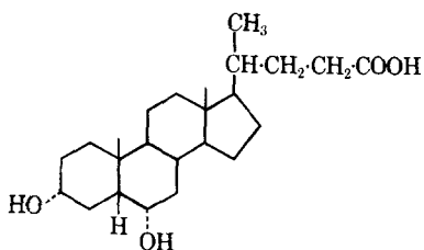
41. Hyodeoxycholic acid
