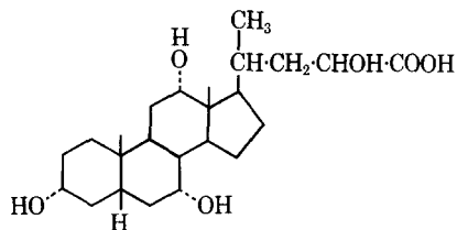
36. 3\alpha,7\alpha,12\alpha,23\xi -Tetrahydroxy- 5\beta -cholanoic acid
