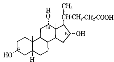
33. Pythocholic acid
