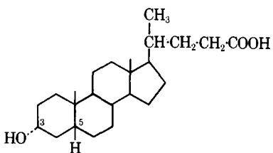
14. Lithocholic acid
