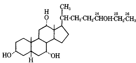
31. 26-Deoxy-5 \beta -ranol
